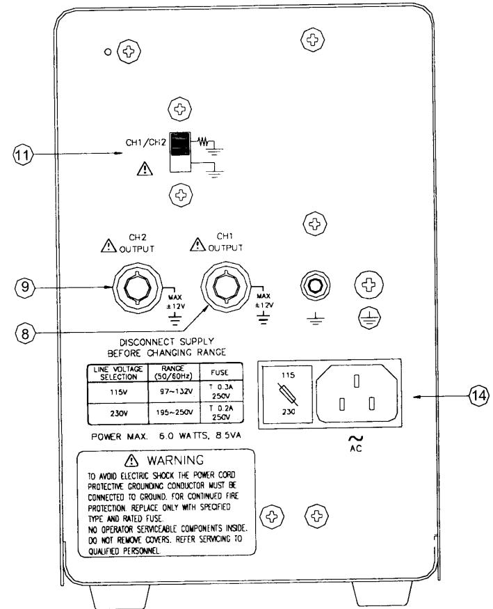
Rear Panel
